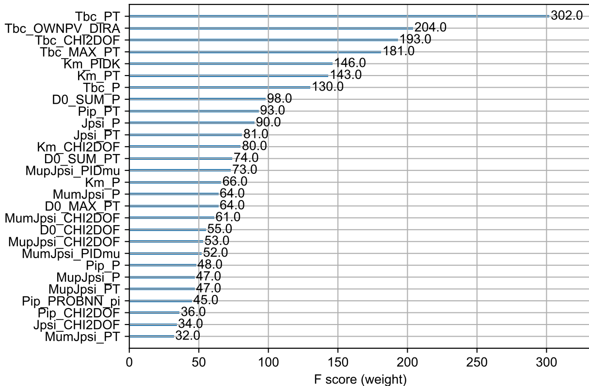
Feature importance
