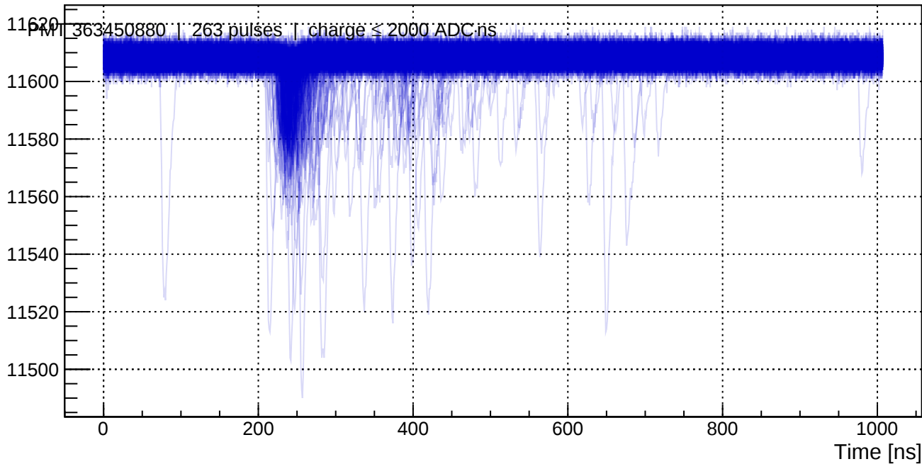
PMT 363450880 -- 263 fired pulses (charge \leq 2000.0 ADC·ns, threshold=15.0 ADC)
