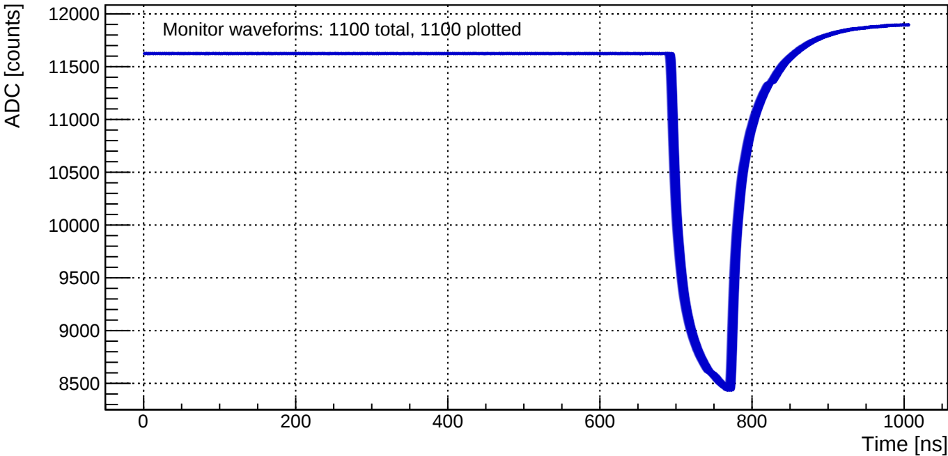
CdMonitorWaveform PMT 43300 -- 1100 pulses (amplitude < 1000000000 ADC)
