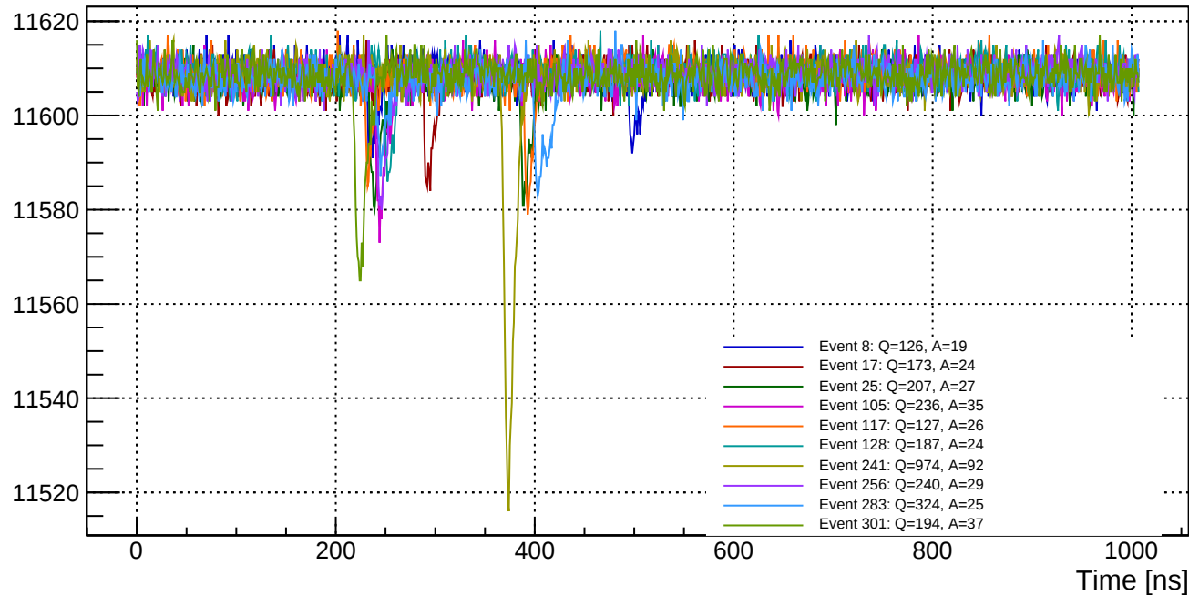
PMT 363450880 " 10 fired pulses (threshold=15 ADC)
