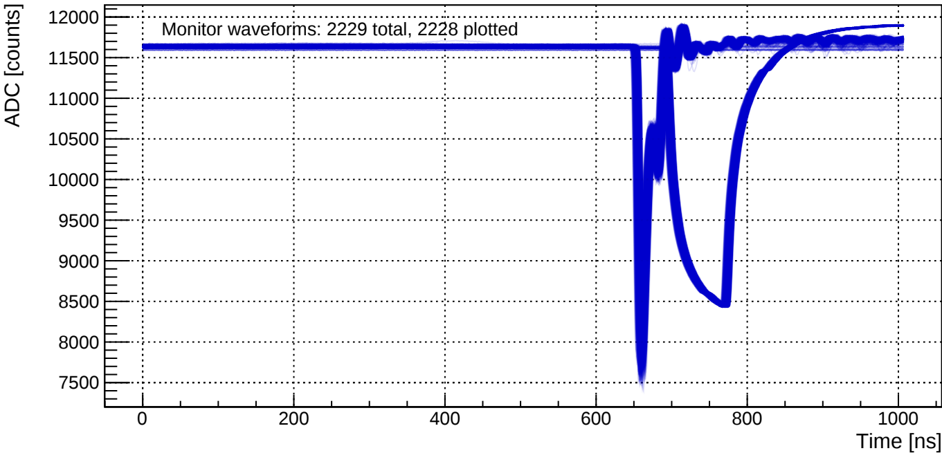
CdMonitorWaveform -- 2228 pulses (amplitude < 6000 ADC)
