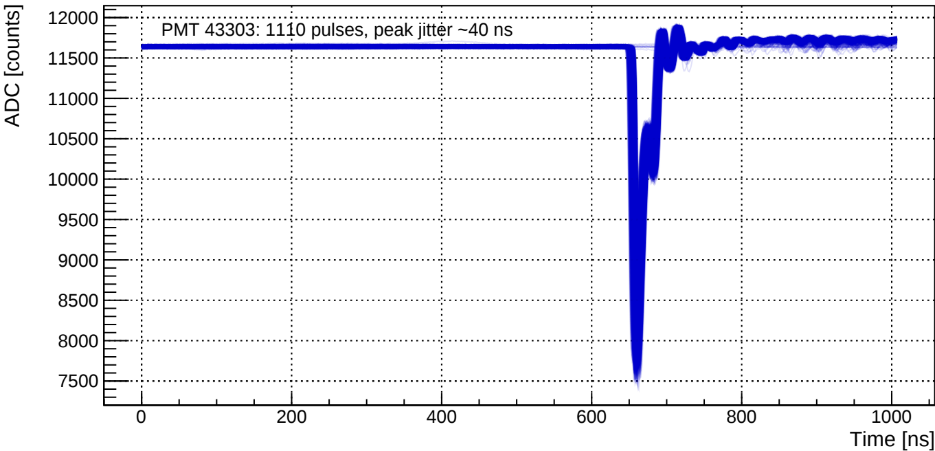
CdMonitorWaveform PMT 43303 -- 1110 pulses
