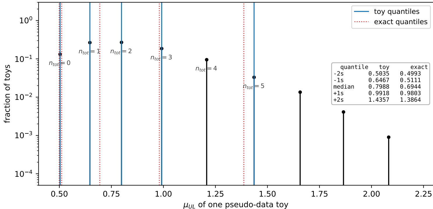
Per-toy upper limits, b -only ensemble ( 10^4 toys, s_1 = s_2 = 3 , b = 1/\text{bin} )
