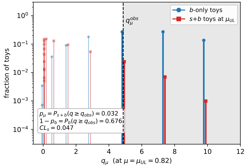
(a) q_\mu distributions and the two tails
