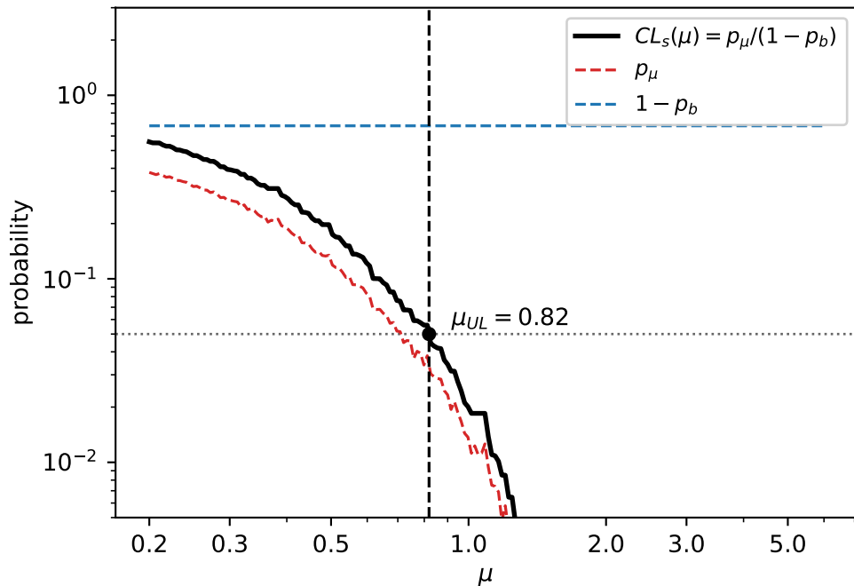
(b) toy CL_s(\mu) scan for n_{obs} = (1, 1)
